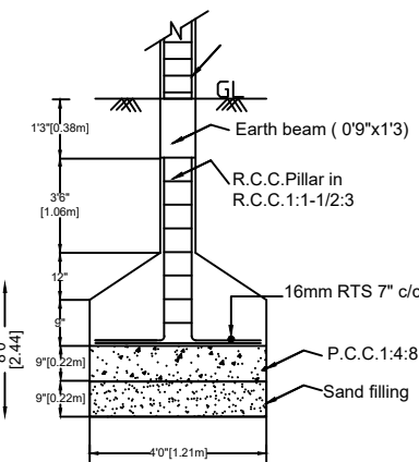
FOUNDATION DETAILS
