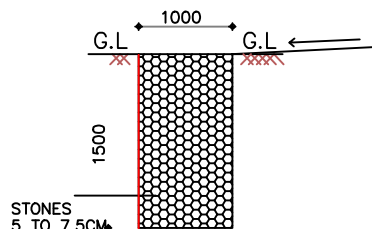
SECTION OF PEBBLE TRENCH
