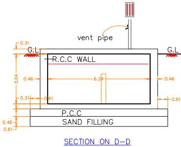
SECTION ON D-D
