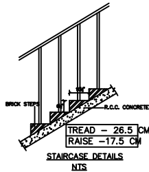
STAIRCASE DETAILS
