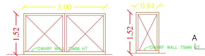
MAIN GATE WICKET GATE
