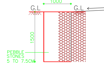
SECTION OF PEBBLE TRENCH SCALE : 1: = 100
