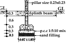
FOUNDATION DETAILS
