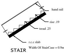
STAIR
