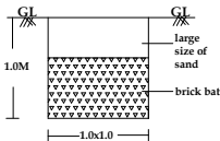
RAINWATER HARVESTING
