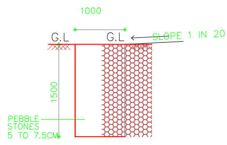
SECTION OF PEBBLE TRENCH SCALE : 1: = 100
