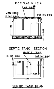
SEPTIC TANK PLAN
