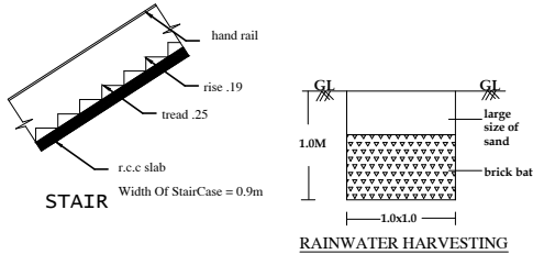
RAINWATER HARVESTING
