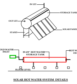
SOLAR HOT WATER SYSTEM DETAILS
