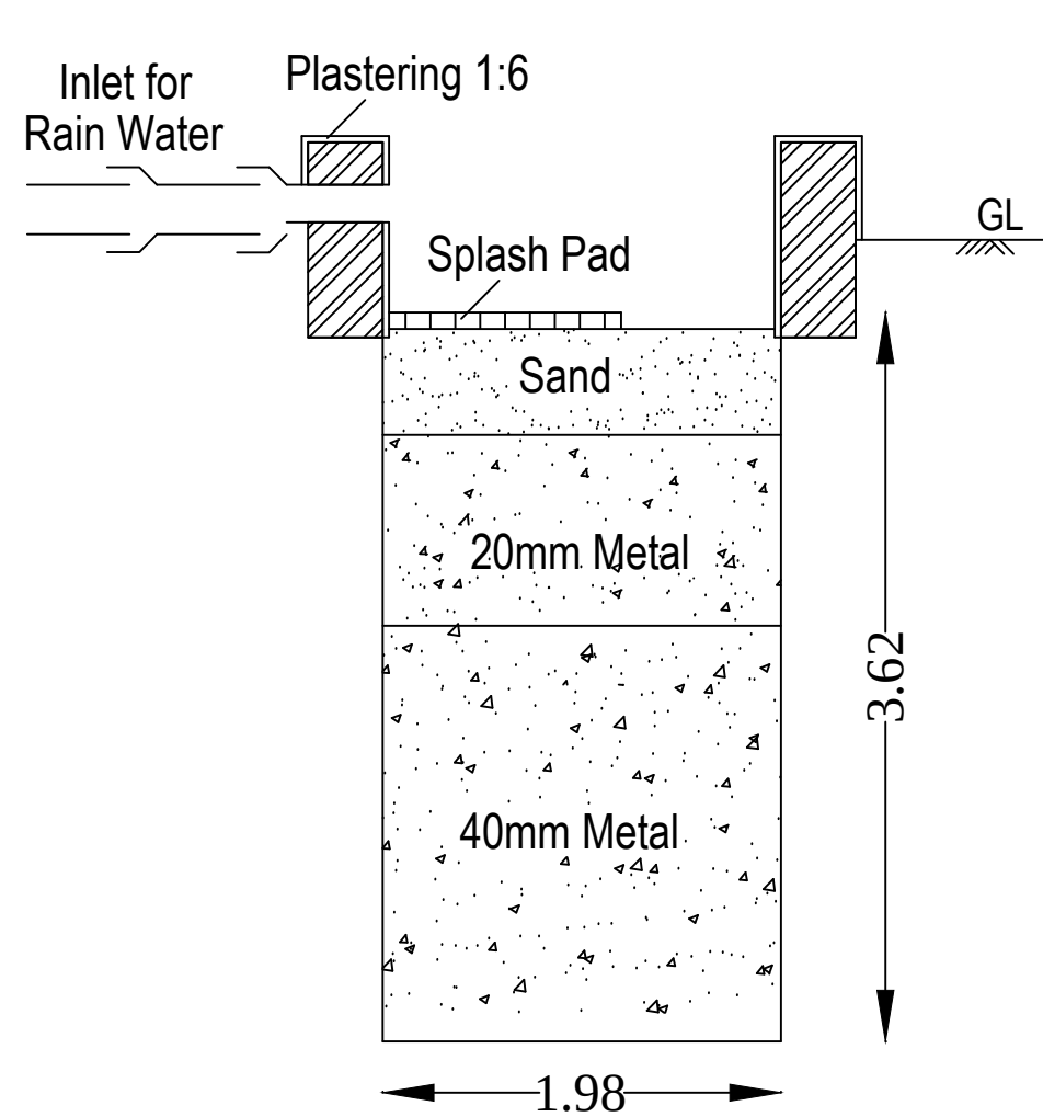
RAIN WATER PERCOLATION PIT
