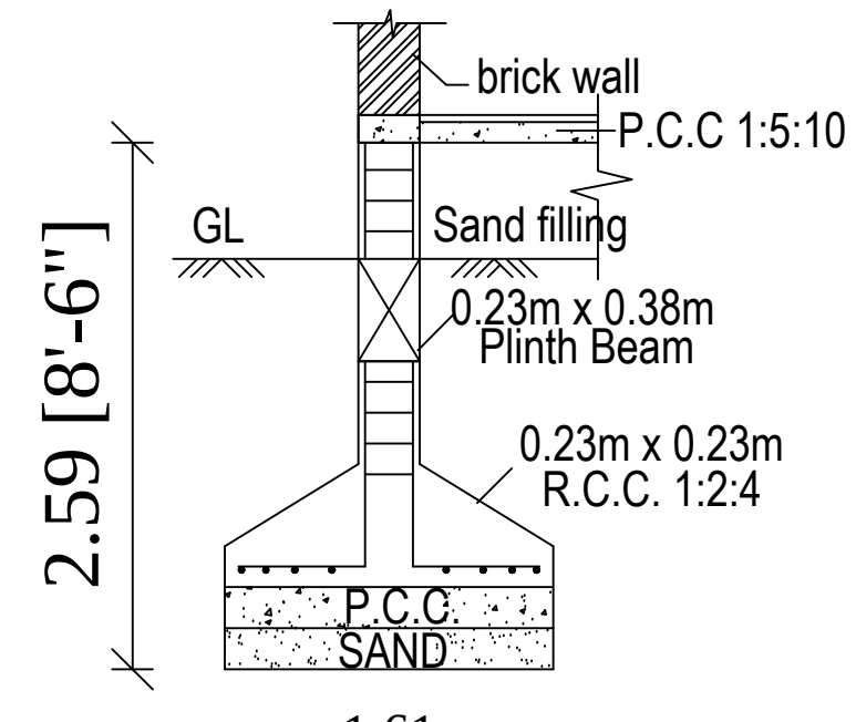
FOUNDATION DETAILS
