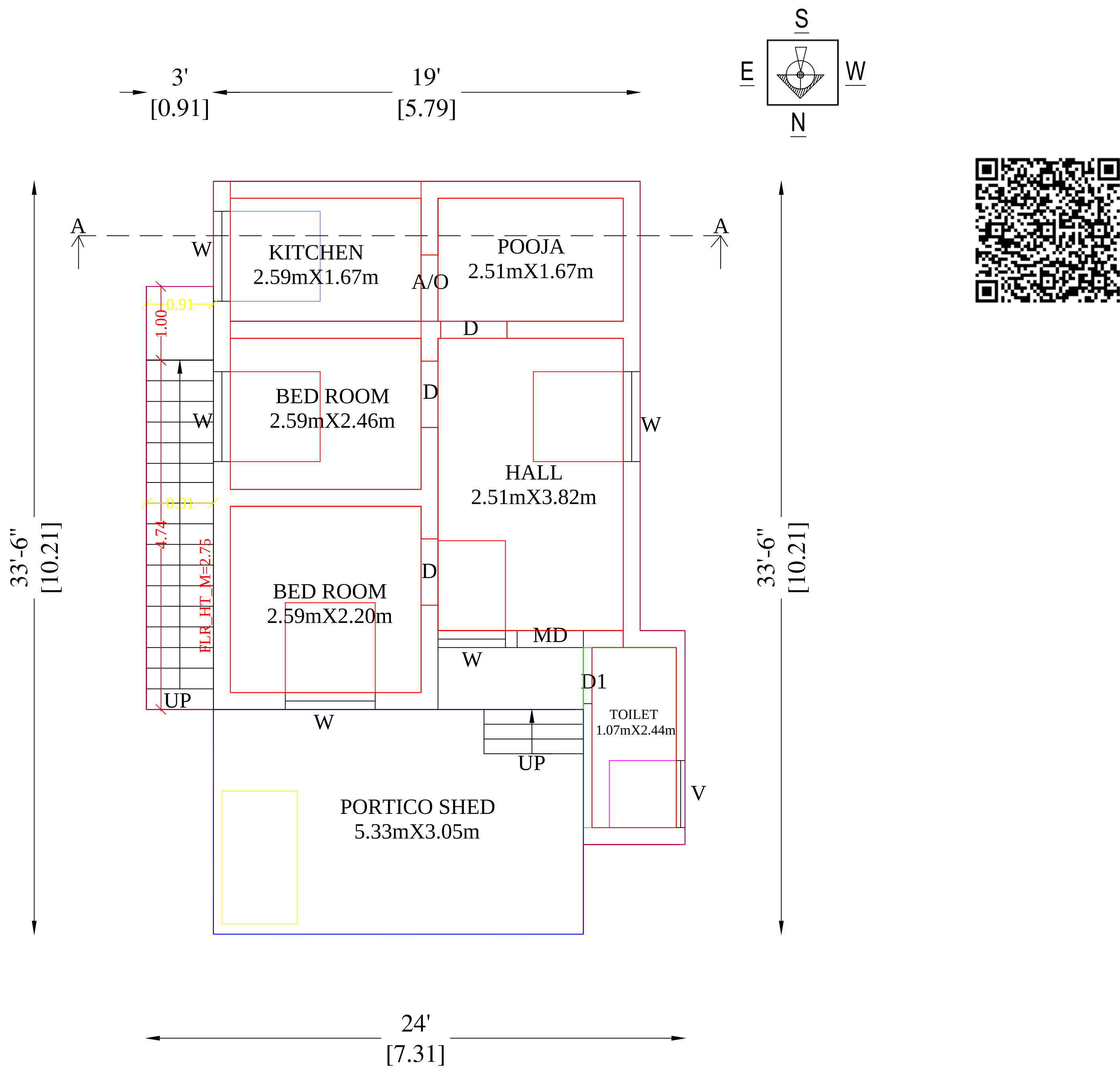
PRO. GROUND FLOOR PLAN
