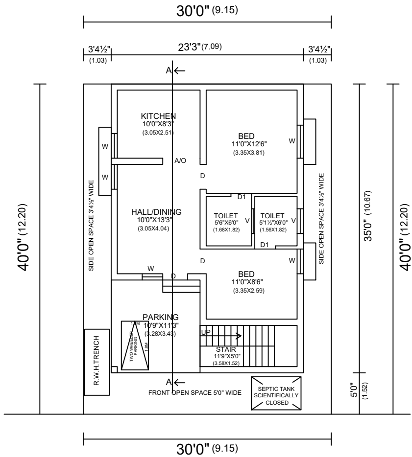
20'0" WIDE ROAD GROUND FLOOR PLAN (PROPOSED)
