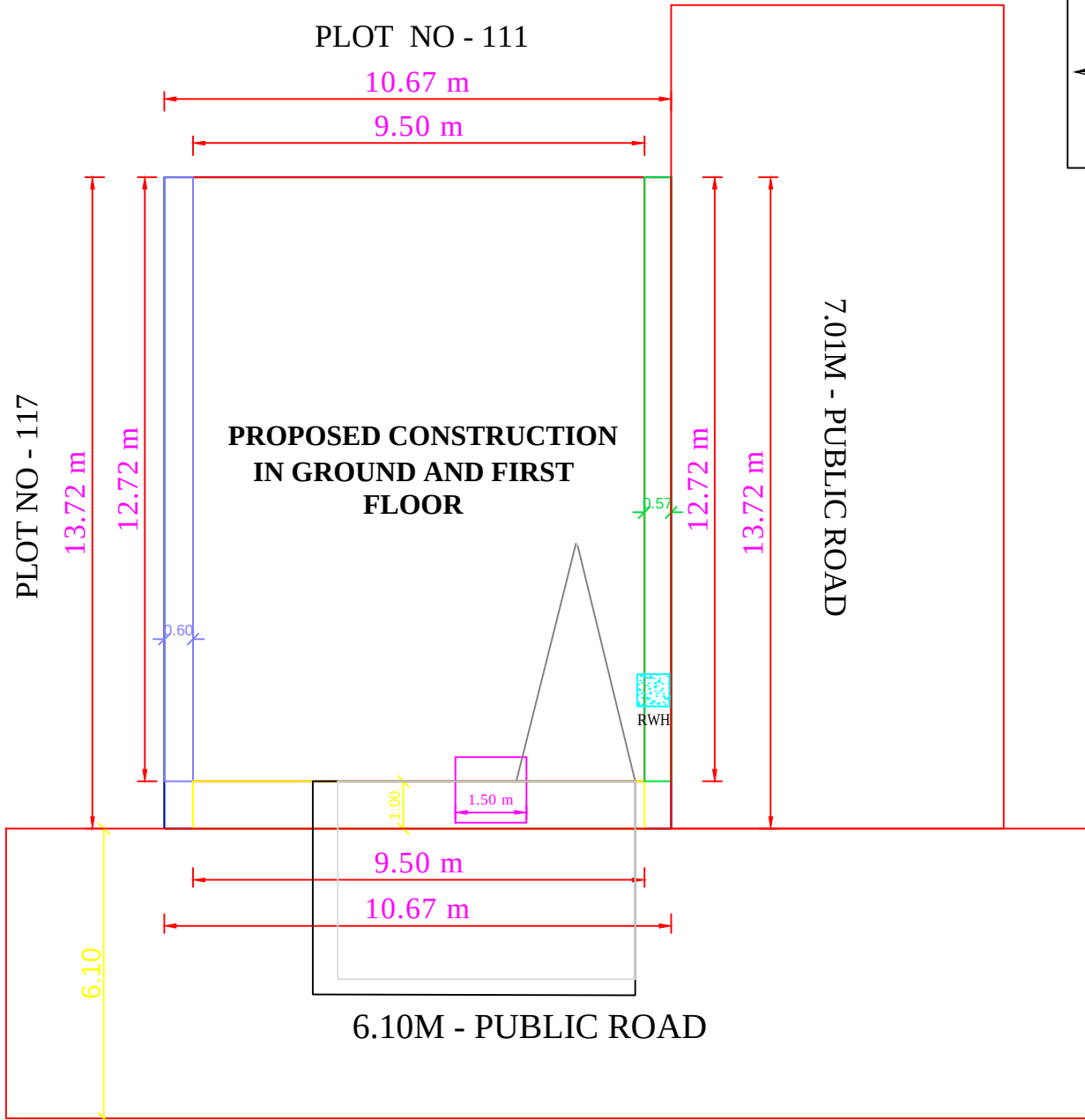
SITE PLAN
