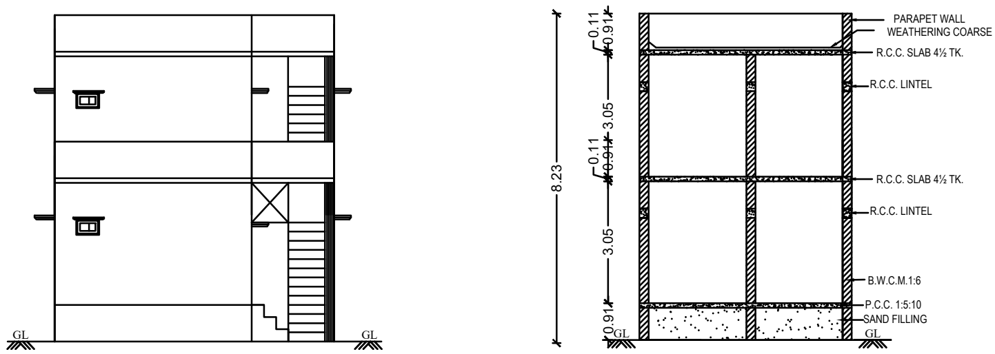
FRONT ELEVATION ( NORTH FACING)
