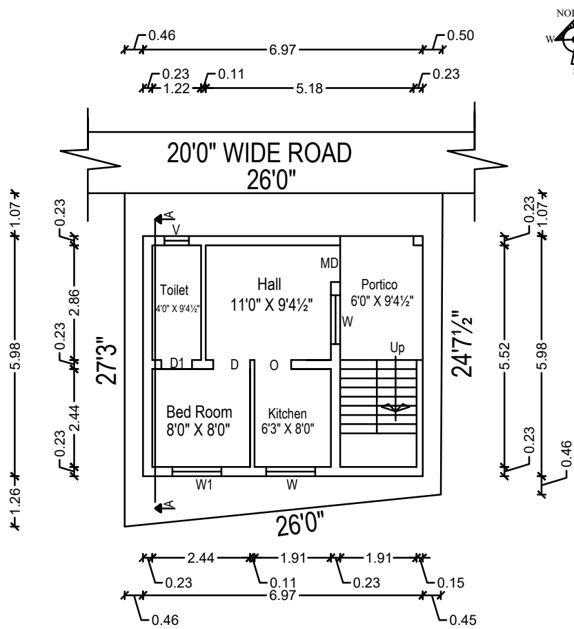
SITE&GROUND FLOOR PLAN
