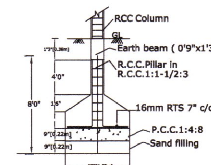
FOUNDATION DETAILS
