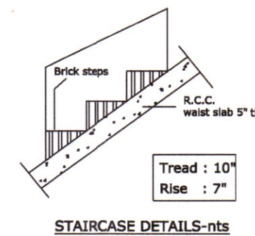
STAIRCASE DETAILS-nts
