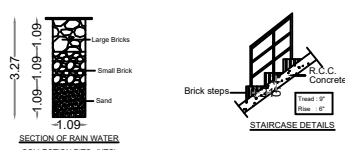
SECTION OF RAIN WATER COLLECTION PITS (NTS)
