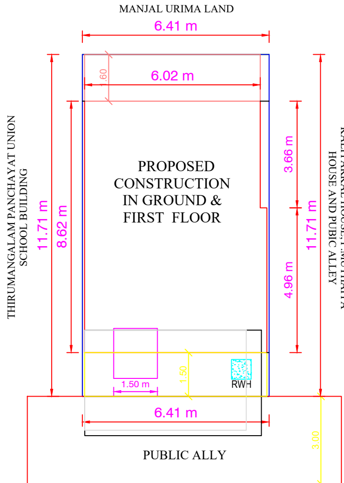
SITE PLAN
