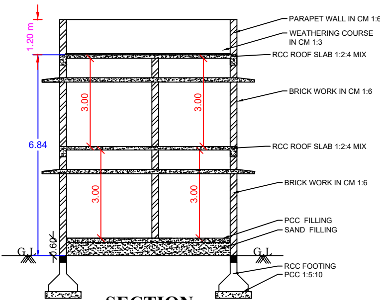
SECTION
