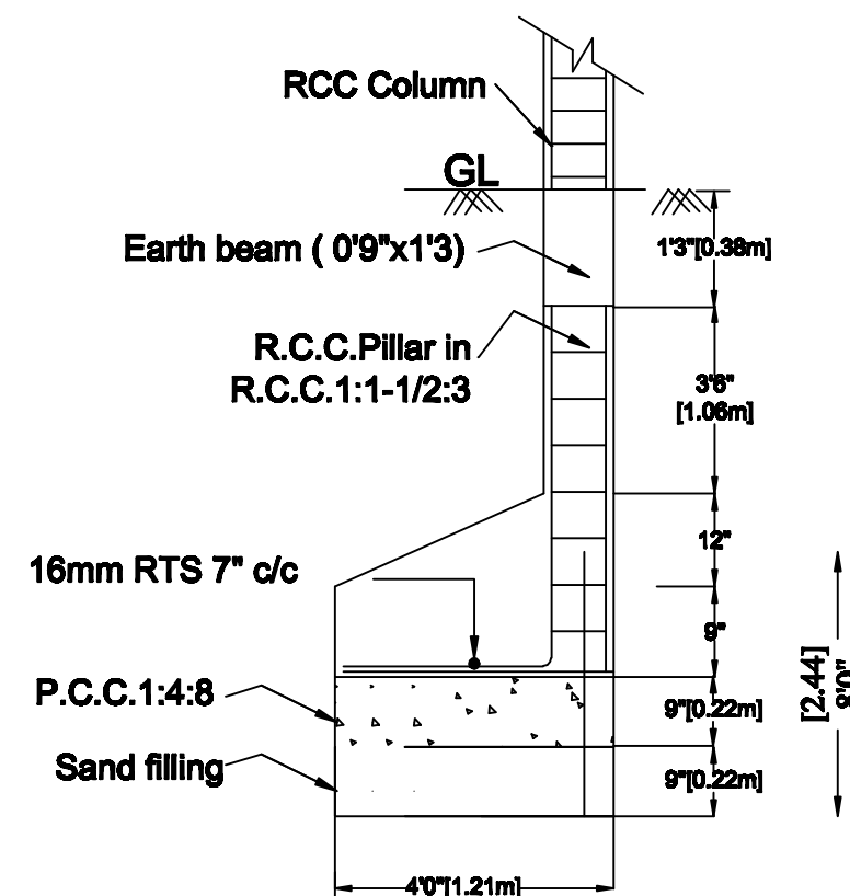
FOUNDATION DETAILS
