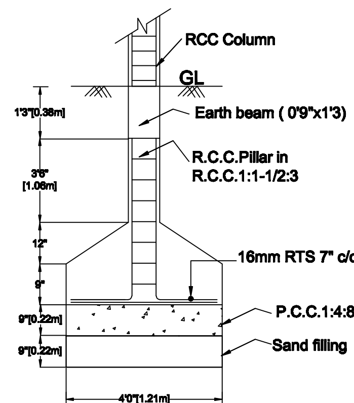
FOUNDATION DETAILS
