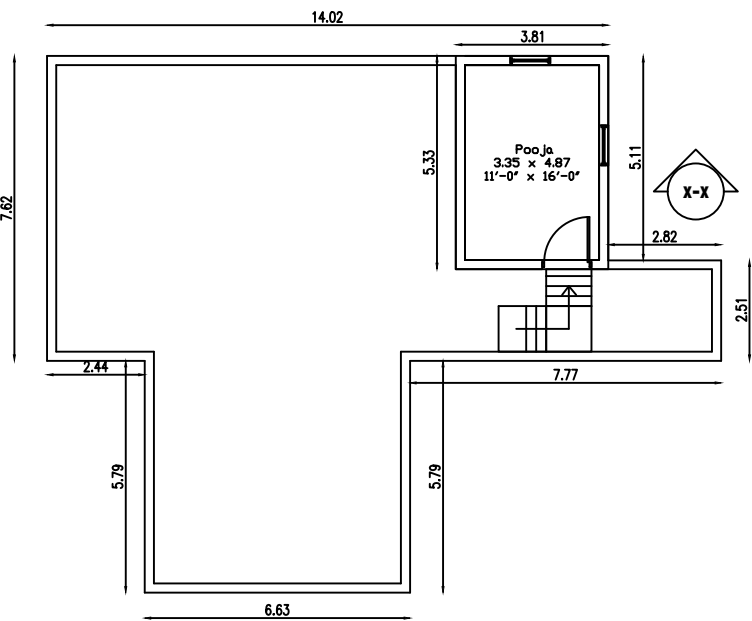
PROPOSED SECOND FLOOR WITH TERRACE FLOOR
