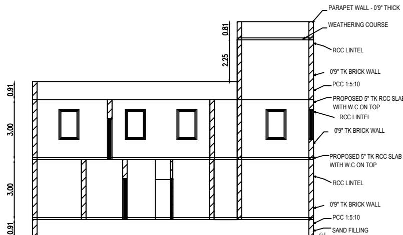
SECTION CUTTING XX
