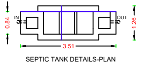
SEPTIC TANK DETAILS-PLAN
