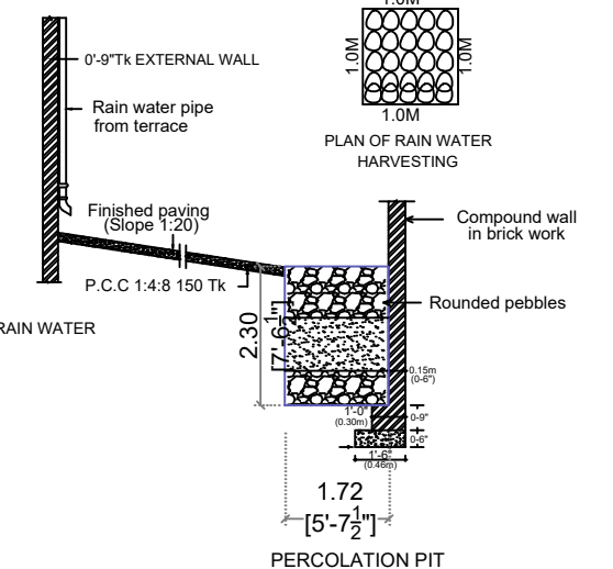
PERCOLATION PIT
