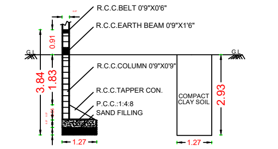
FOUNDATION DETAILS-END COLUMN
