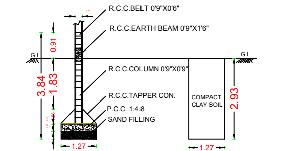
FOUNDATION DETAILS-MIDDLE COLUMN
