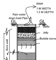
SEC. RAIN WATER HARVEST PIT
