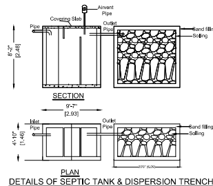
DETAILS OF SEPTIC TANK & DISPERSION TRENCH
