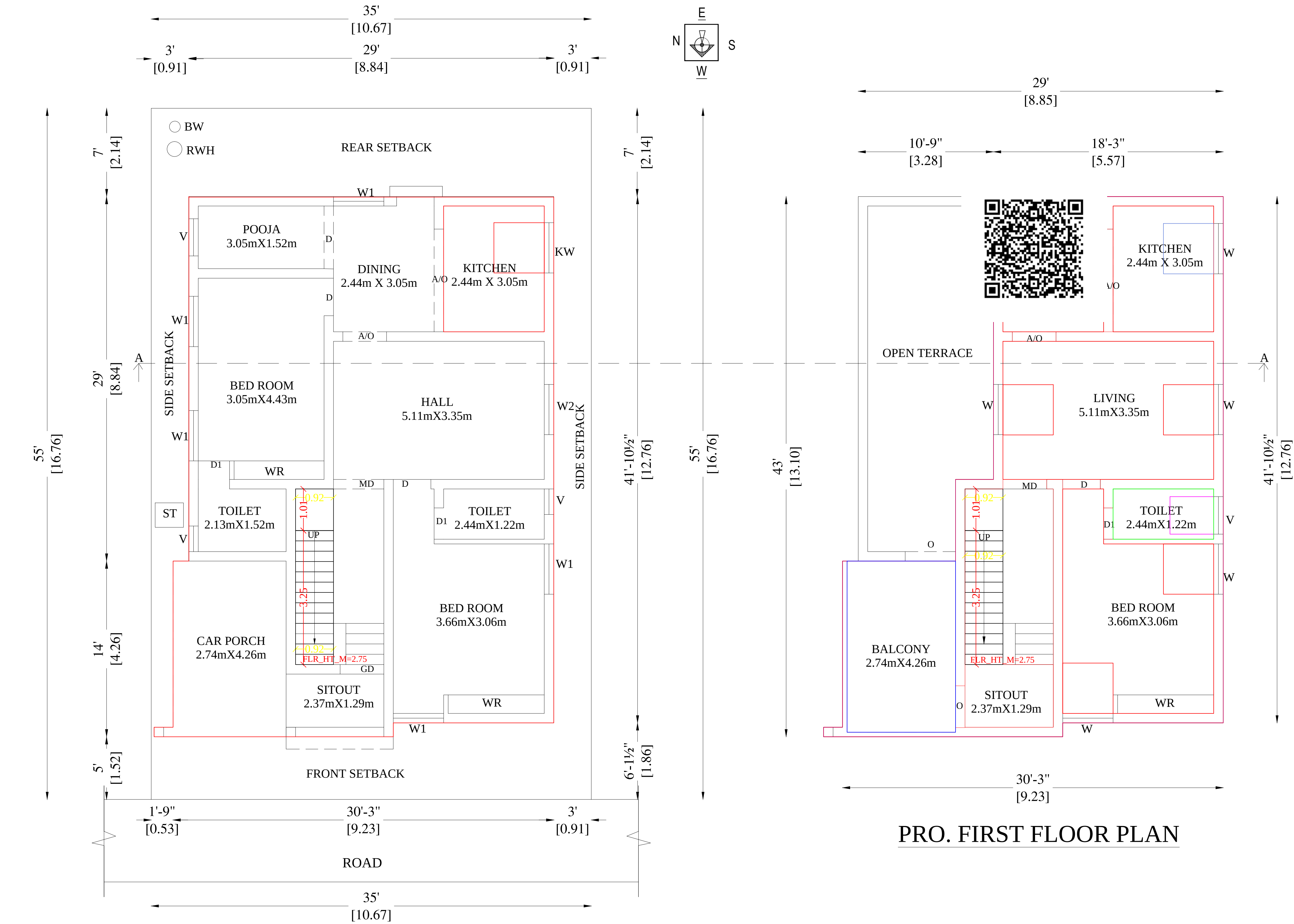
EXG. GROUND FLOOR PLAN
