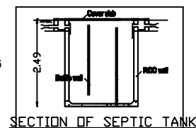
SECTION OF SEPTIC TANK
