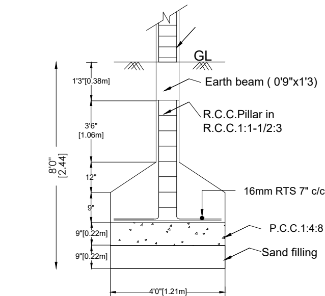
FOUNDATION DETAILS
