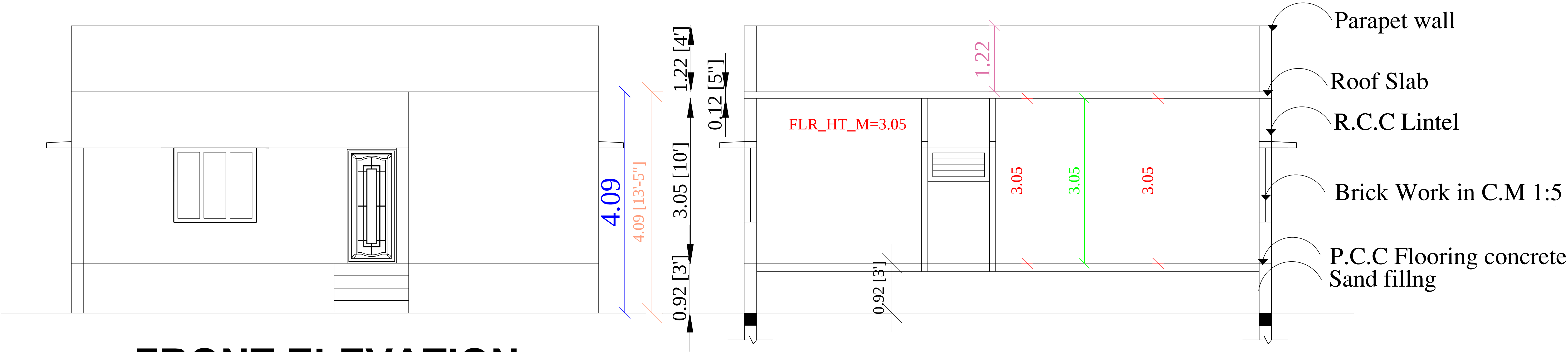
SECTION ON"AA"
