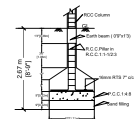
FOUNDATION DETAILS
