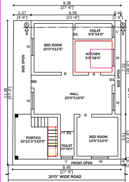
EXG. GROUND FLOOR PLAN
