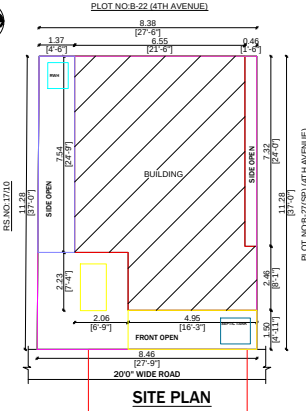
SITE PLAN
