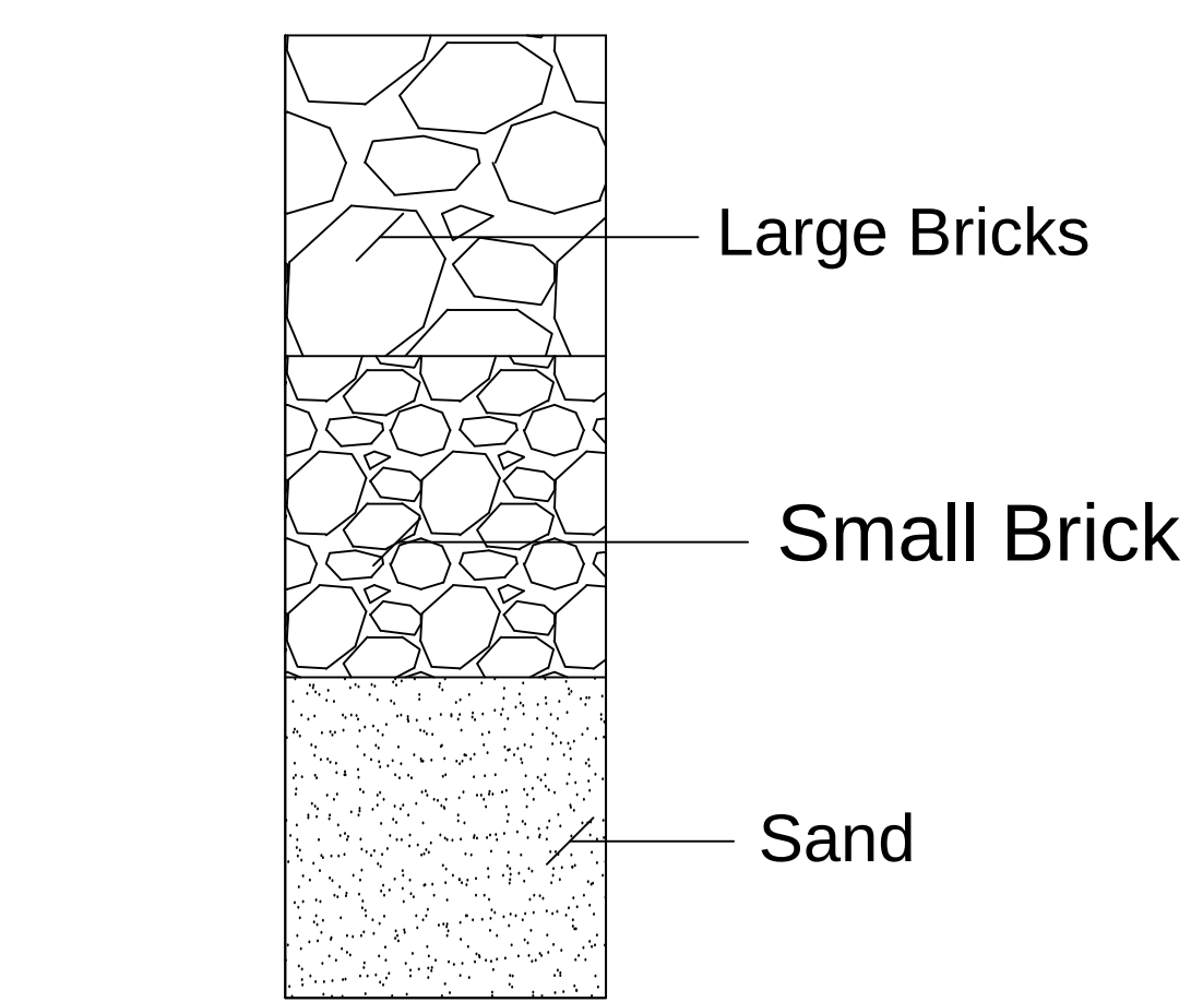
SECTION OF RAIN WATER COLLECTION PITS (NTS)
