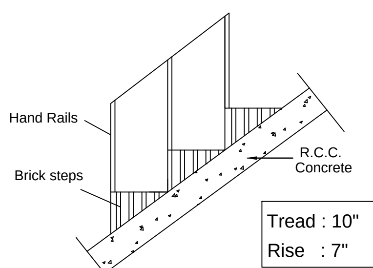
STAIRCASE DETAILS
