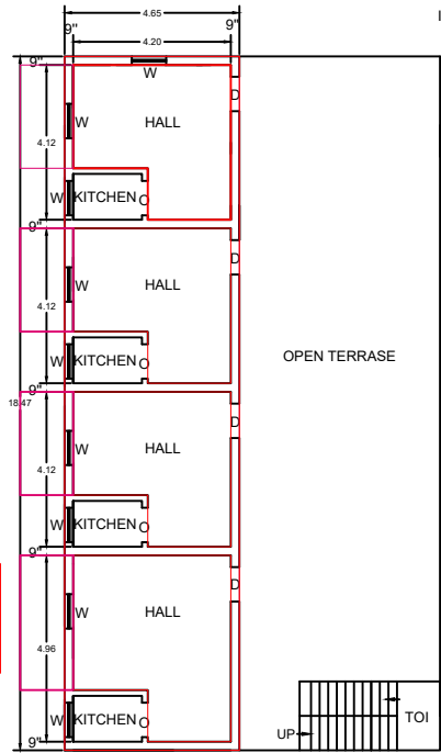
PROPOSED S.F. PLAN
