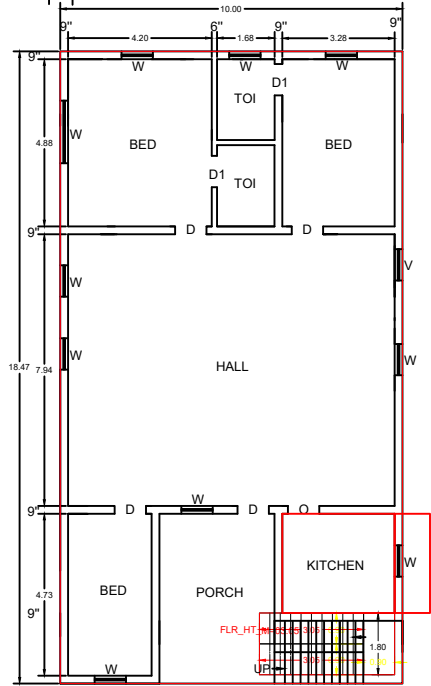
EXISTING F.F. PLAN
