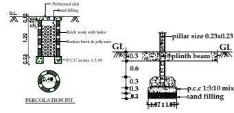
FOUNDATION DETAILS
