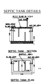
SEPTIC TANK PLAN
