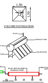
SOLAR HOT WATER SYSTEM DETAILS
