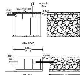
DETAILS OF SEPTIC TANK & DISPERSION TRENCH
