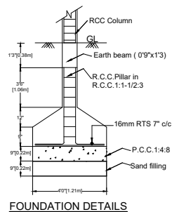
FOUNDATION DETAILS
