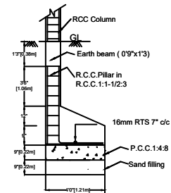
FOUNDATION DETAILS
