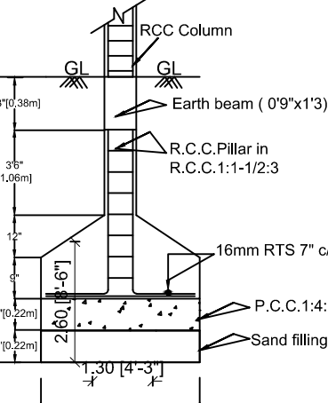
FOUNDATION DETAILS
