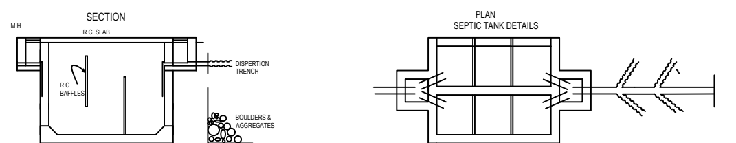
DETAILS OF SEPTIC TANK
