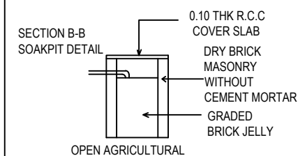
DETAILS OF SOAK PIT
