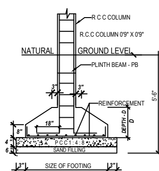
TYPICAL FOOTING DETAILS
