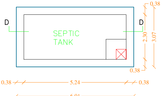
PLAN OF SEPTIC TANK SCALE 1"-2'0"
