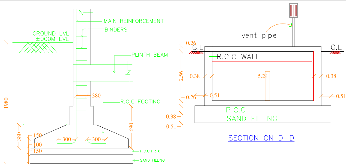
TYPICAL SECTION OF R.C.C COLUMN FOUNDATION SCALE : 1" = 2'-0"
