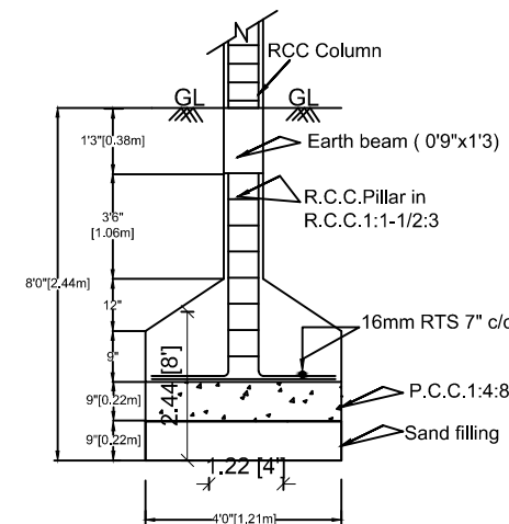
FOUNDATION DETAILS
