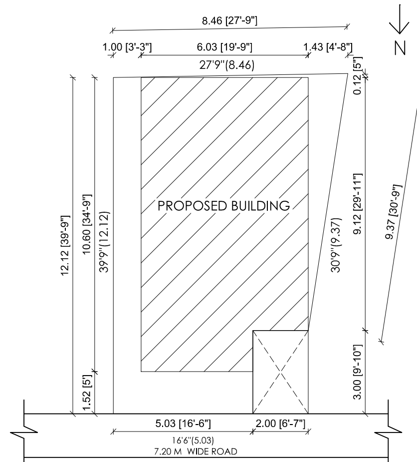
SITE PLAN
