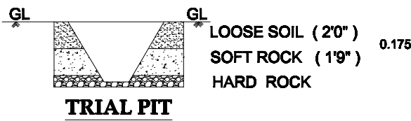
TRIAL PIT
