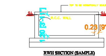
RWH_CAPACITY_L = 2000LTRS
