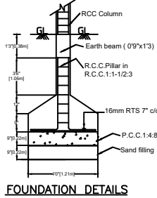
FOUNDATION DETAILS
