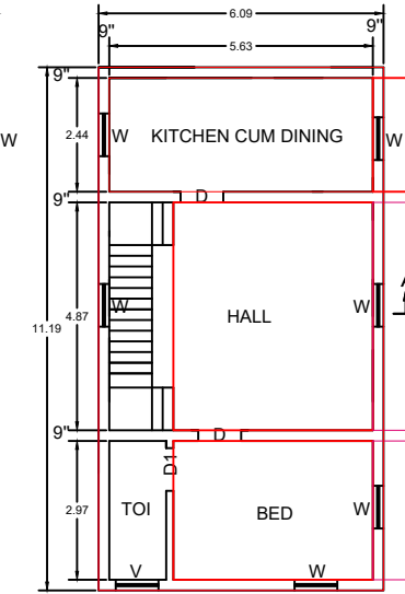
PROPOSED S.F. PLAN
