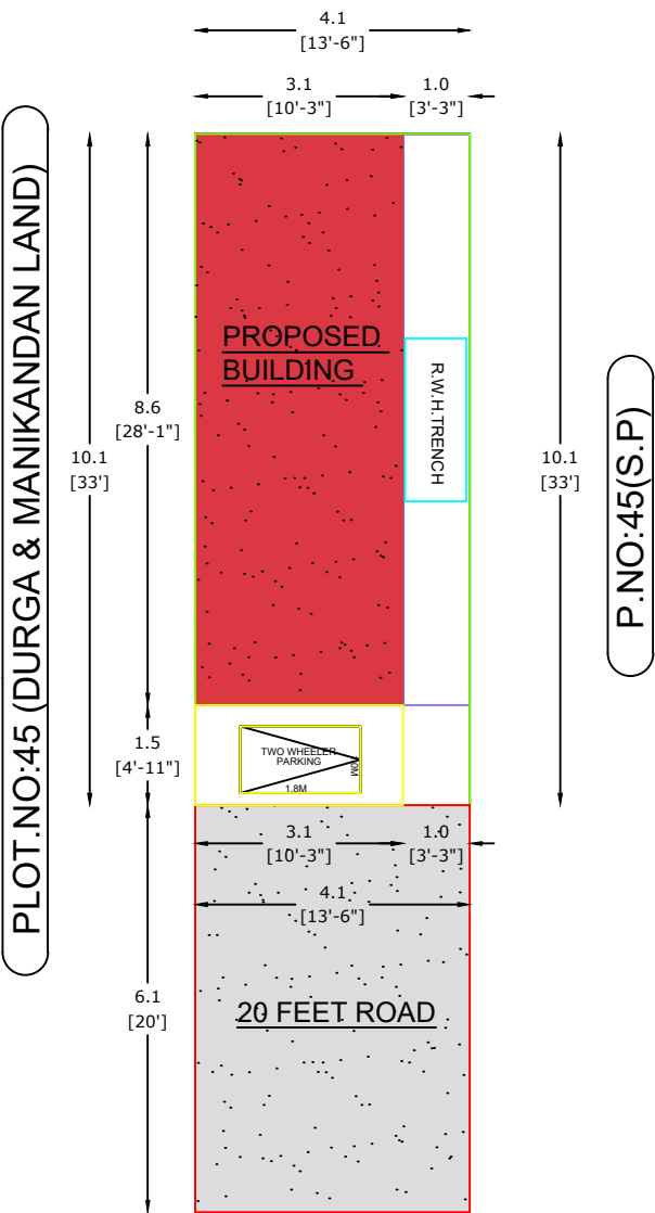
SITE PLAN
