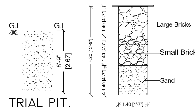
SECTION OF RAIN WATER COLLECTION PITS (NTS)
