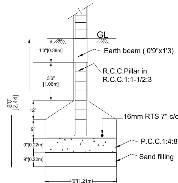
FOUNDATION DETAILS
