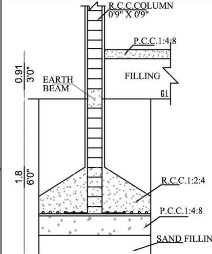
FOUNDATION DETAILS NOT TO SCALE
