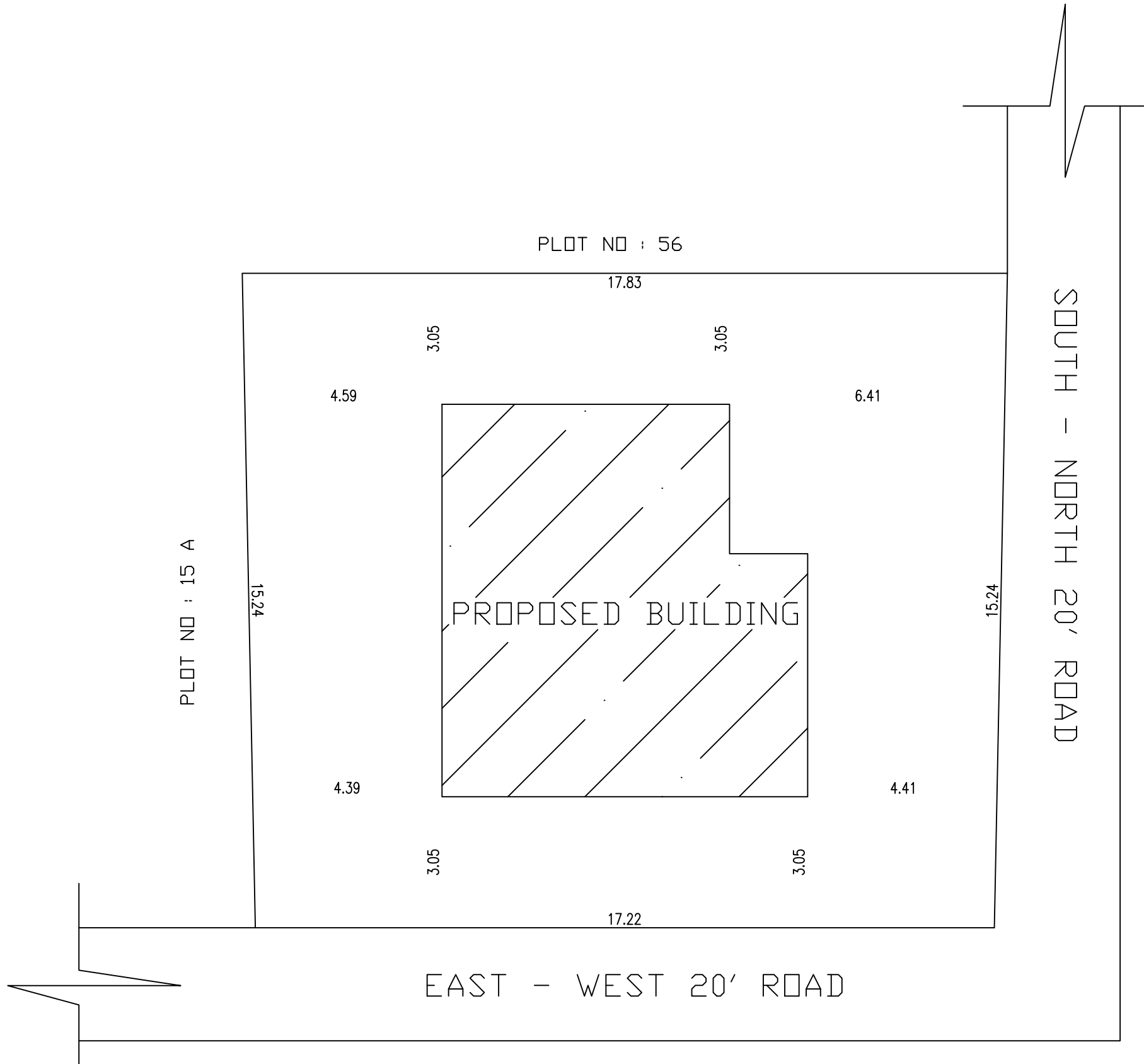
SITE PLAN AS PER SCALE
