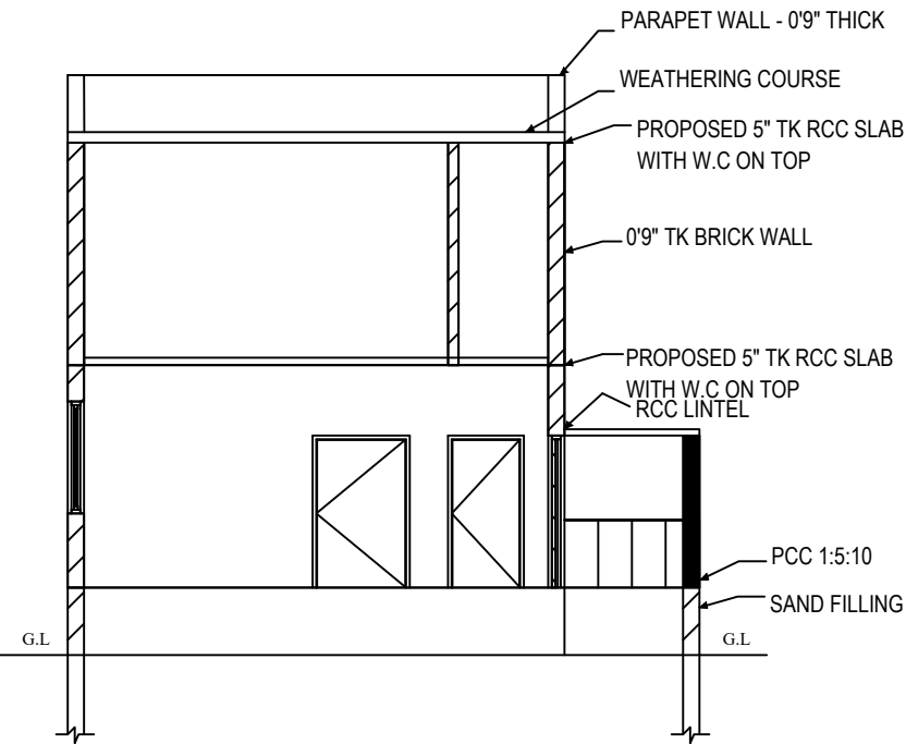
SECTION CUTTING XX
