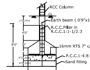
FOUNDATION DETAILS
