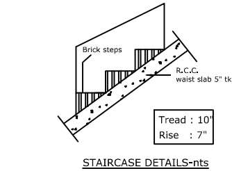
STAIRCASE DETAILS-nts
