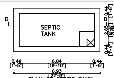
PLAN OF SEPTIC TANK SCALE 1"=2'0"
