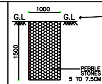
SECTION OF PEBBLE TRENCH SCALE : 1: = 100
