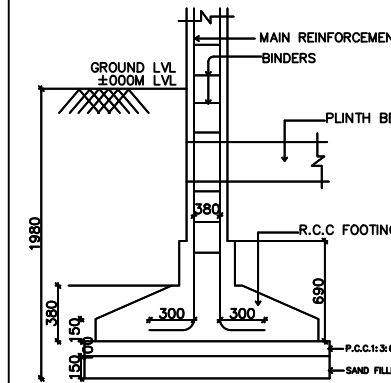
TYPICAL SECTION OF R.C.C COLUMN FOUNDATION
