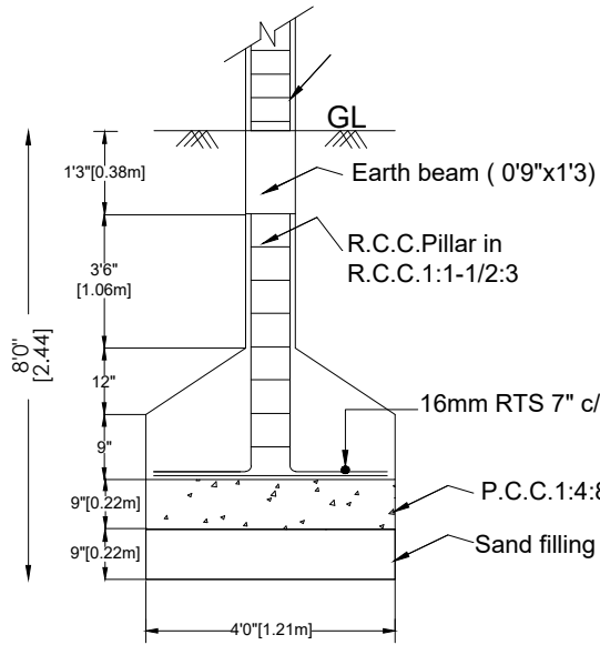
FOUNDATION DETAILS
