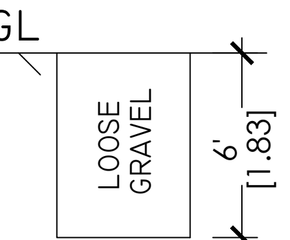
TRIAL PIT.
