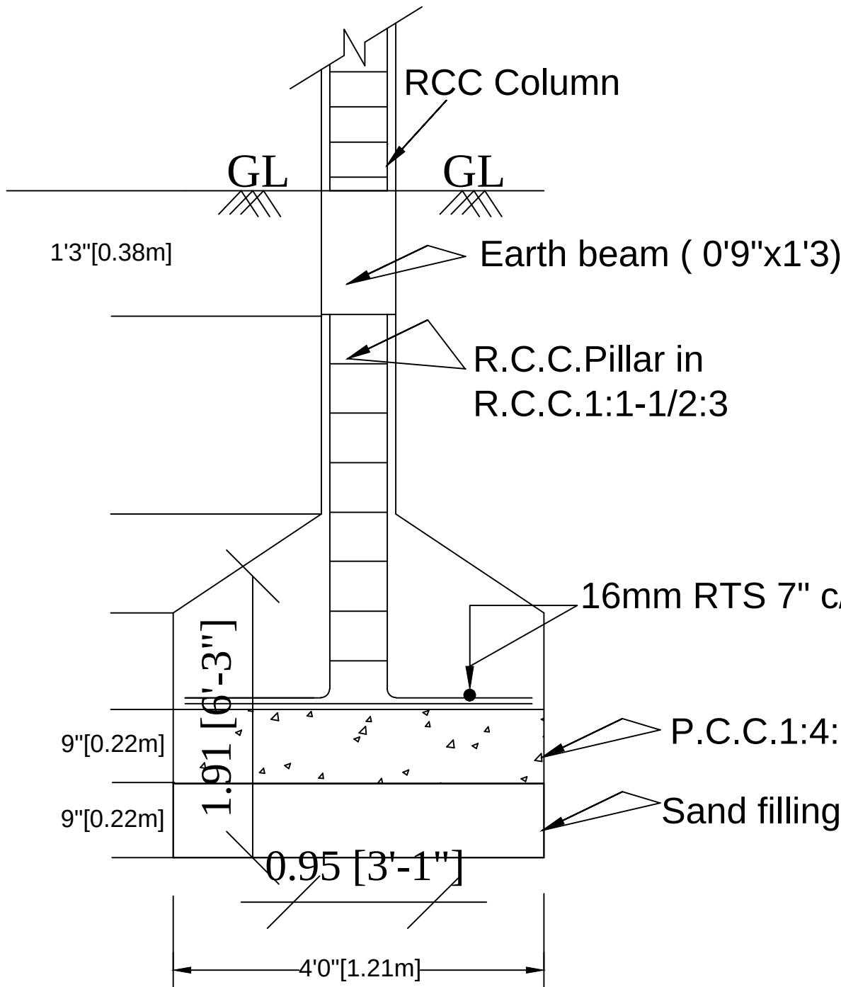
FOUNDATION DETAILS
