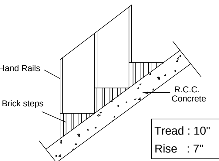
STAIRCASE DETAILS
