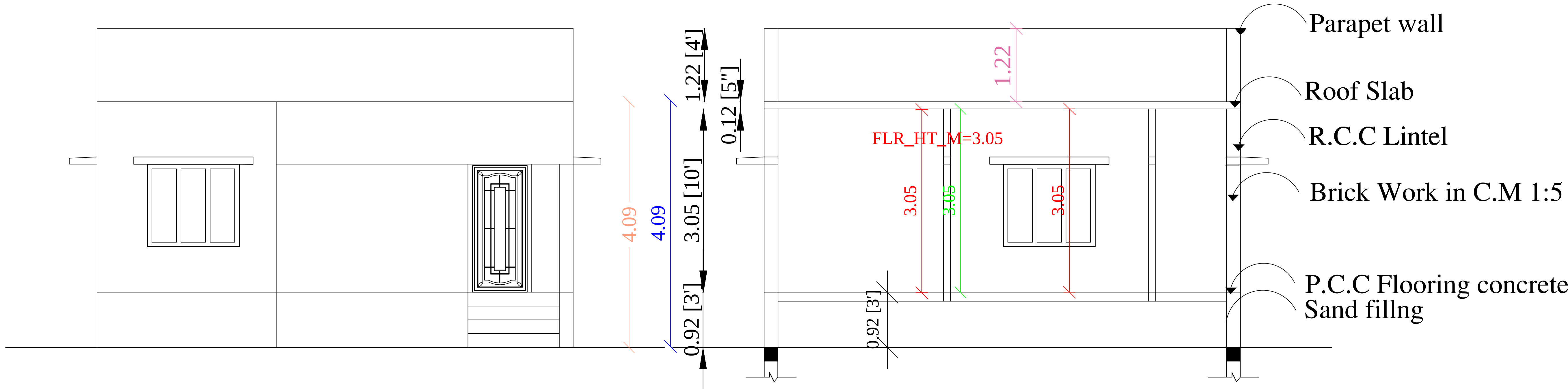
FRONT ELEVATION
