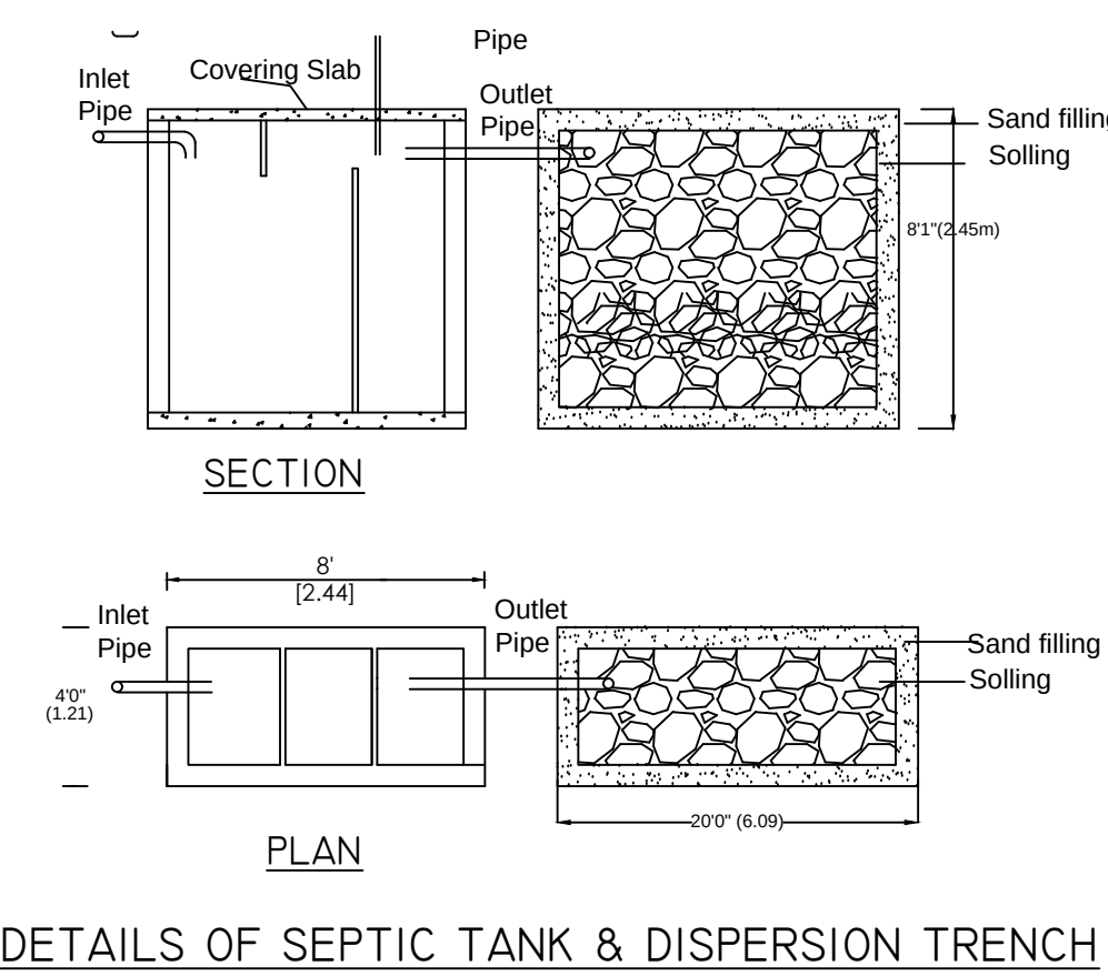
DETAILS OF SEPTIC TANK & DISPERSION TRENCH
