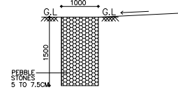
SECTION OF PEBBLE TRENCH SCALE : 1 = 100
