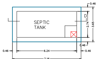
PLAN OF SEPTIC TANK SCALE 1\"/>
