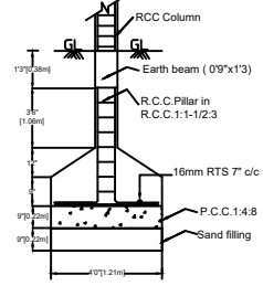
FOUNDATION DETAILS
