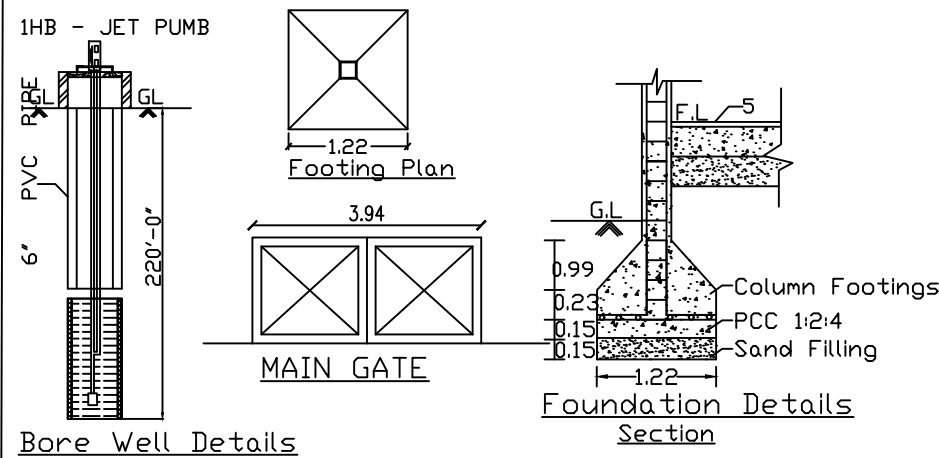
Bore Well Details
