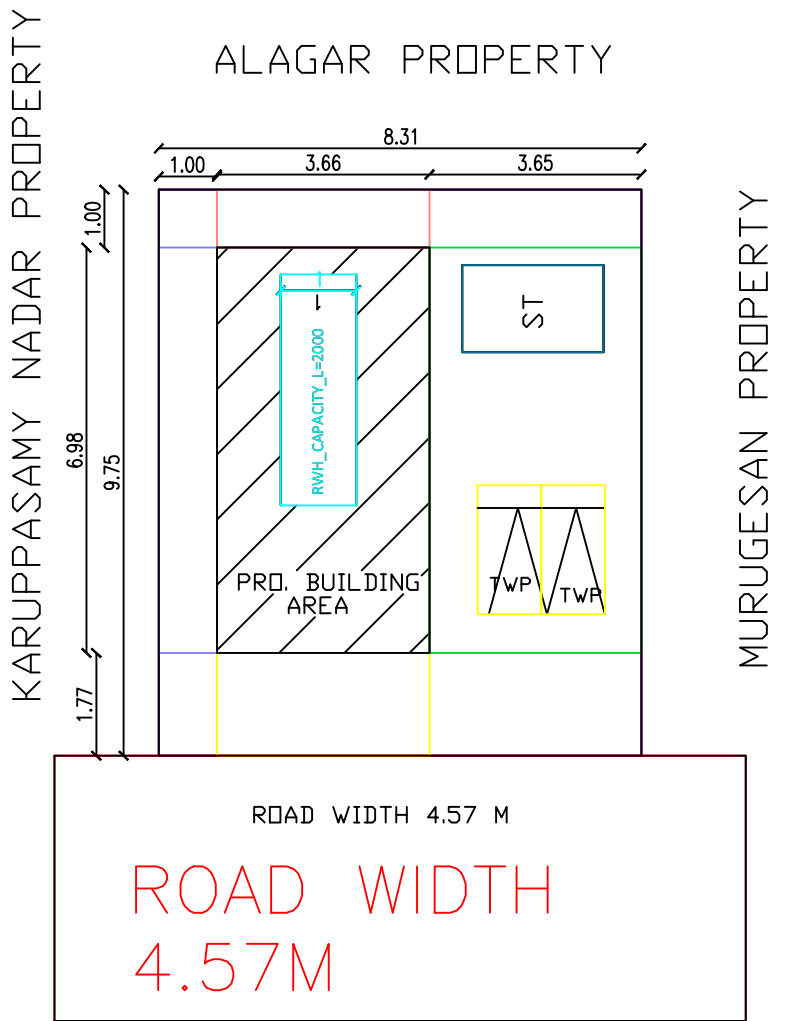
SITE PLAN
