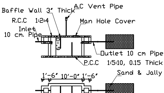
Septic Tank with Dispersion Trench
