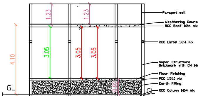
SECTION ON "VR"
