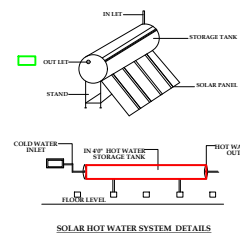
SOLAR HOT WATER SYSTEM DETAILS
