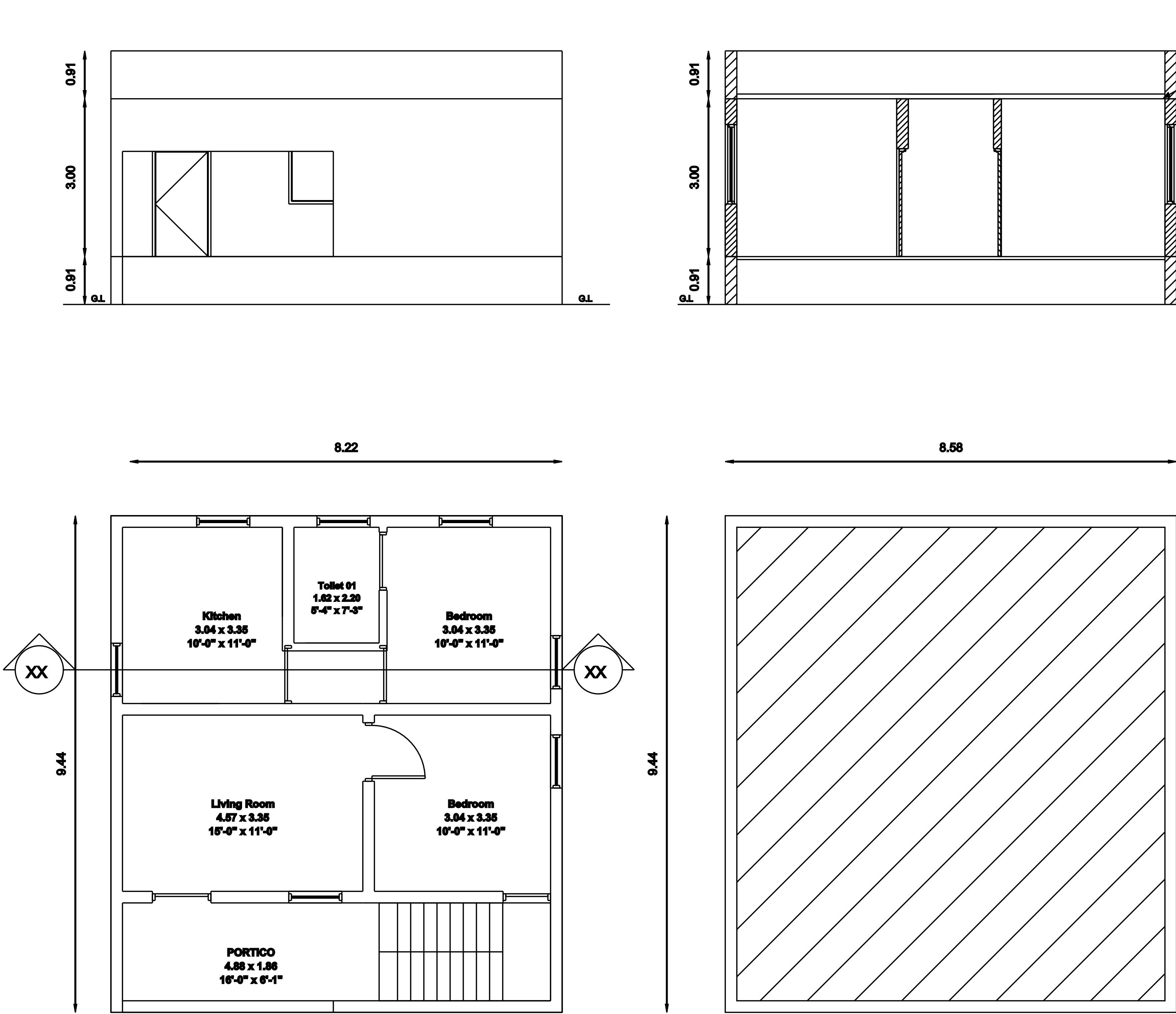
TERRACE FLOOR
