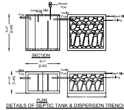
DETAILS OF SEPTIC TANK & DISPERSION TRENCH
