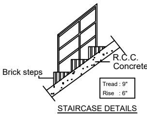
STAIRCASE DETAILS
