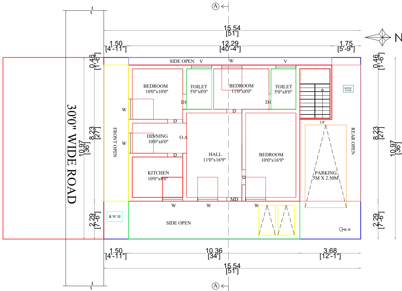
G .GROUND FLOOR PLAN
